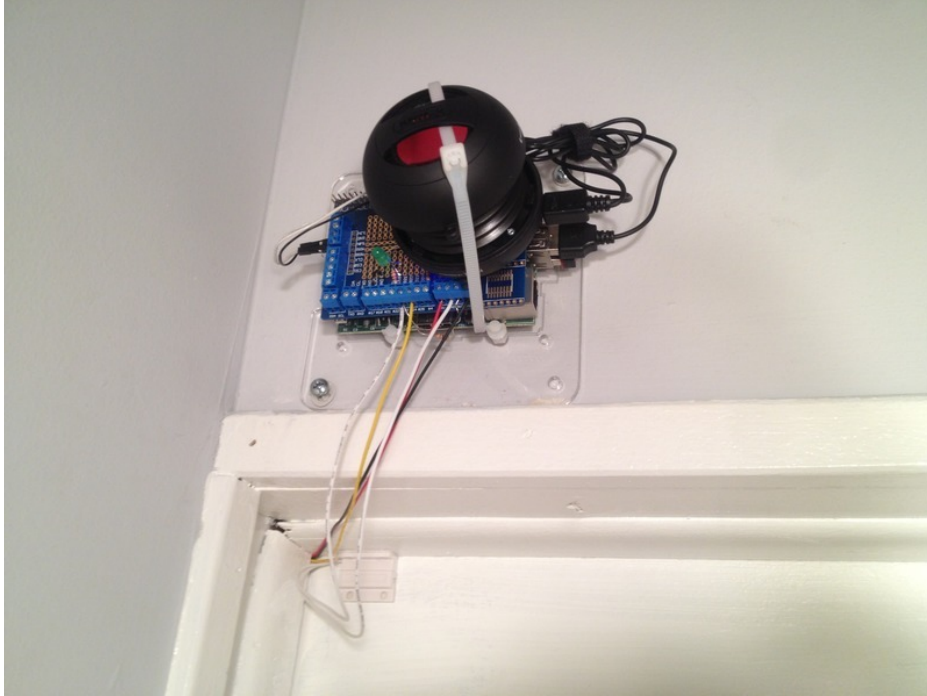
Pi, Pi plate, and speaker all stacked together on the VESA mount above the door.
