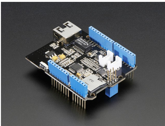
Ethernet Shield for Arduino - W5500 Chipset
