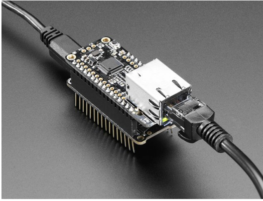
Adafruit Ethernet FeatherWing
