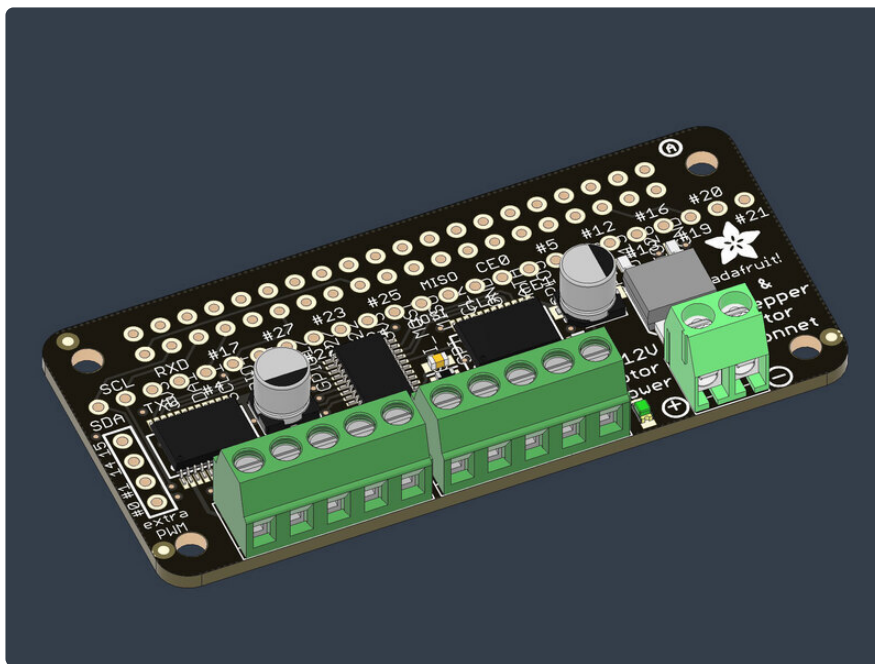
3D model DC Stepper Motor Bonnet
